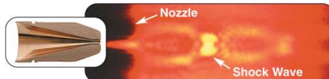
Schlieren image showing density gradients clearly identifies a Mach Disc (shock wave) present in the gas flow as it exits from a traditionally manufactured laser nozzle.
